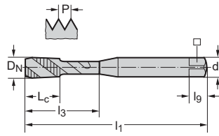
Steam Oxide or TiAlN * Semi-Bottoming * DIN Length with ANSI Shank
