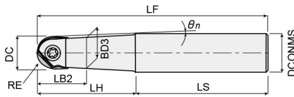
Type A (Taper neck)
