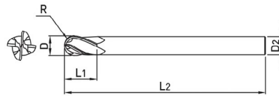
CORNER RADIUS 4 FLUTE END MILL WITHOUT REACH - INCH
