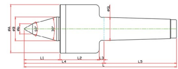
NC HIGH SPEED ROTATIONAL- MINIMIZES BITE INTERFERENCE- LIVE CENTER
