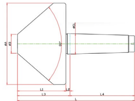
PT-80 - PIPE MACHINING - HOLLOW NOSE - LIVE CENTER
