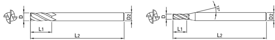
CORNER RADIUS 4 FLUTE END MILL WITHOUT REACH - INCH
