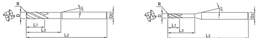
CORNER RADIUS - 4 FLUTE, EXTENDED NECK with 1.5XD CUT LENGTH - 30° HELIX - ALTiN+HH Coating - METRIC
