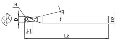
BALL NOSE - 2 FLUTE with NECK - LONG CUT LENGTH, ALTiN COATING - METRIC
