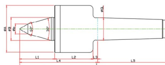
C HIGH SPEED ROTATIONAL - LIVE CENTERS
