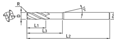
CORNER RADIUS - 4 FLUTE, EXTENDED NECK with 1.5XD CUT LENGTH - 30 ° HELIX - ALTiN+HH Coating - METRIC
