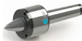
NC HIGH SPEED ROTATIONAL- MINIMIZES BITE INTERFERENCE- LIVE CENTER
