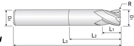
CORNER RADIUS - 5 FLUTE with EXTENDED NECK - REGULAR CUT LENGTH, TiALN+SH COATING - INCH
