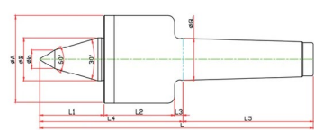
NC HIGH SPEED ROTATIONAL- MINIMIZES BITE INTERFERENCE- LIVE CENTER
