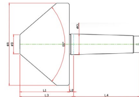
PT-80 - PIPE MACHINING - HOLLOW NOSE - LIVE CENTER
