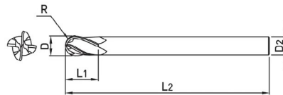
CORNER RADIUS 4 FLUTE END MILL WITHOUT REACH - INCH
