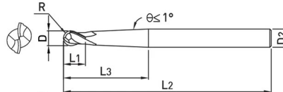
BALL NOSE - 2 FLUTE with PENCIL NECK - SHORT CUT LENGTH, ALTiN COATING - INCH
