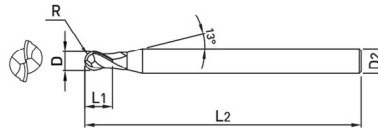
BALL NOSE - 2 FLUTE with NECK - REGULAR & LONG LENGTHS - TiALN+SH - METRIC
