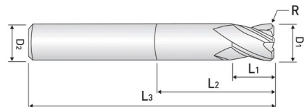
CORNER RADIUS - 5 FLUTE with EXTENDED NECK & SHANK - REGULAR CUT LENGTH, TiALN+SH COATING - INCH
