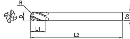
BALL NOSE - 4 FLUTE - VARIABLE HELIX - CUT LENGTH 5XD, TiALN+SH COATING - INCH
